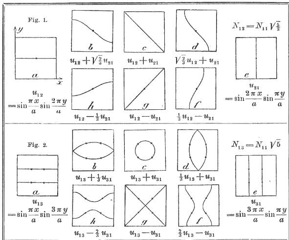
Figure: Nodal sets, Dirichlet eigenvalues \lambda_2 and \lambda_5 (Pockels, [32]).
